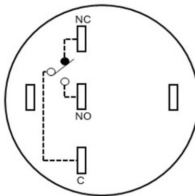
SPDT SWITCH DIAGRAM
